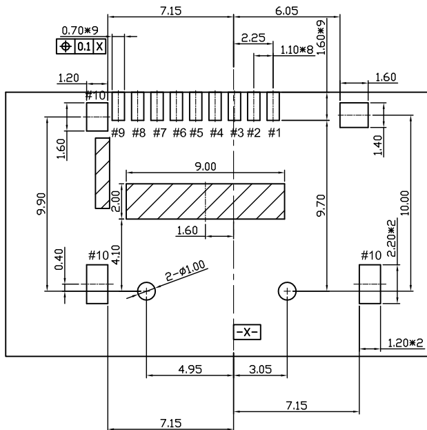
RECOMMENDED PCB LAYOUT (ALL TOLERANCE ARE ±0.05)
